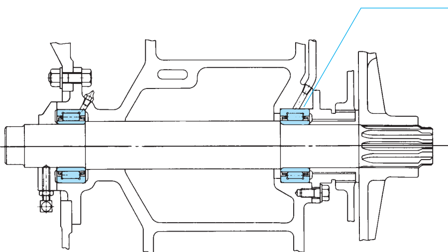
Machined ring needle roller bearings
